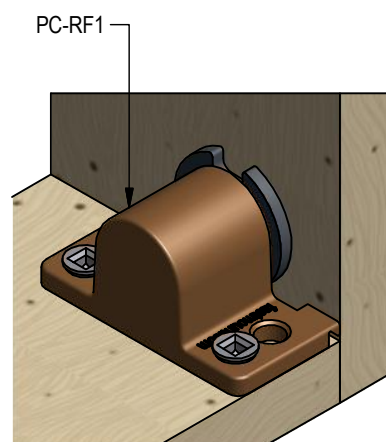
Corner detail at cabinet or shelf
